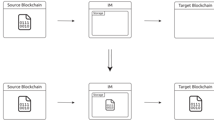
Fig. 7. Data transfer between two DLTs.
