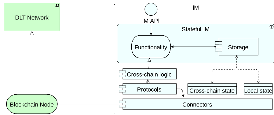
Fig. 5. Representation of a general-purpose blockchain interoperability solution in the Archimate modeling language [122].
