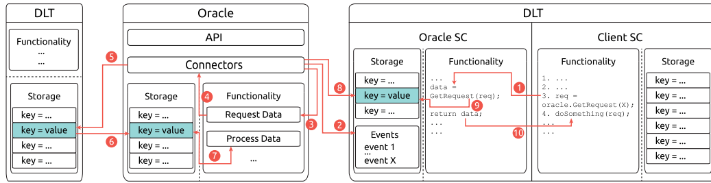
Fig. 10. Pull-based oracle architecture on execute-order-validate (e.g., Ethereum).
