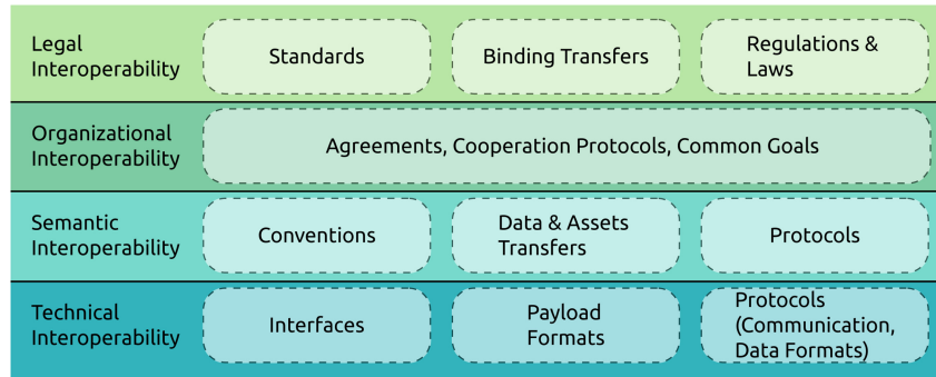
Fig. 4. Interoperability layers (see [44]).
