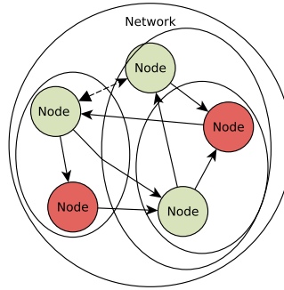
(c) Networks can be organized into subnetworks. Nodes of each subnetwork share a partial view of the distributed ledger. Nodes can be in one or more subnetworks.
