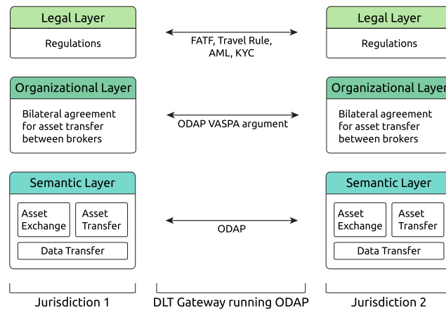
Fig. 14. Example of interoperation between two DLTs connected by a DLT gateway network running a digital asset transfer protocol such as ODAP [60]. A compatibility assessment can be performed regarding the participating DLTs.
