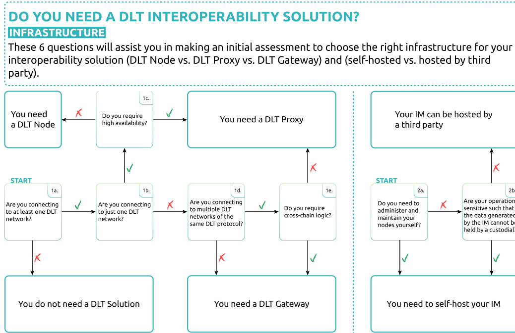
Fig. 15. Decision map guiding the choice of the infrastructure of a DLT interoperability solution. Start on the topmost left node (with the green START label) and answer the questions until you arrive to an end node (blue nodes). The output of this process is a group of IMs that respect the requirements stated on the process flow.
