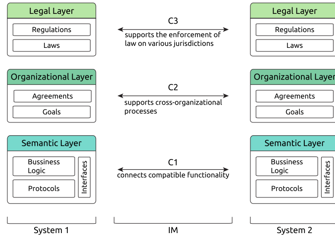
Fig. 13. Compatibility assessment between two systems.
